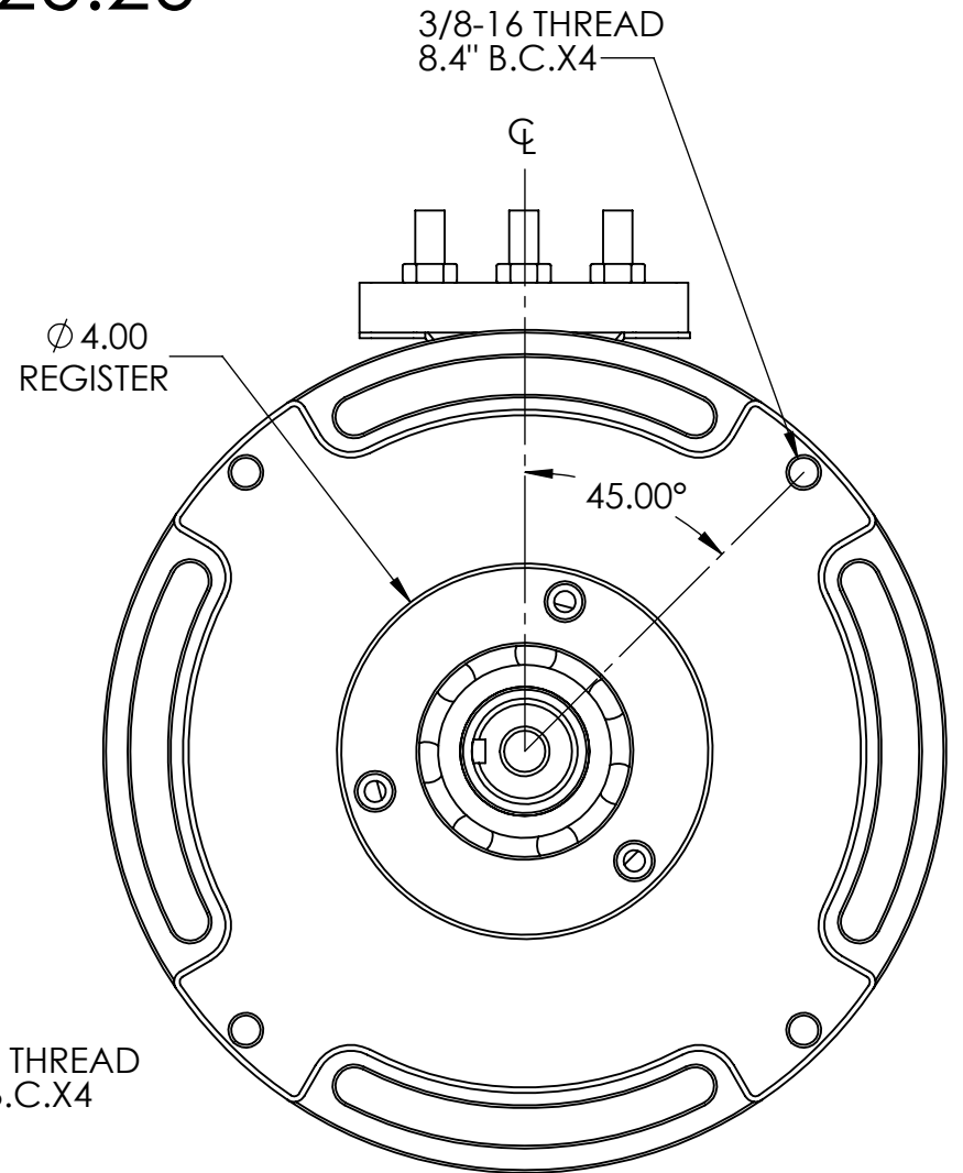
DRIVE END
